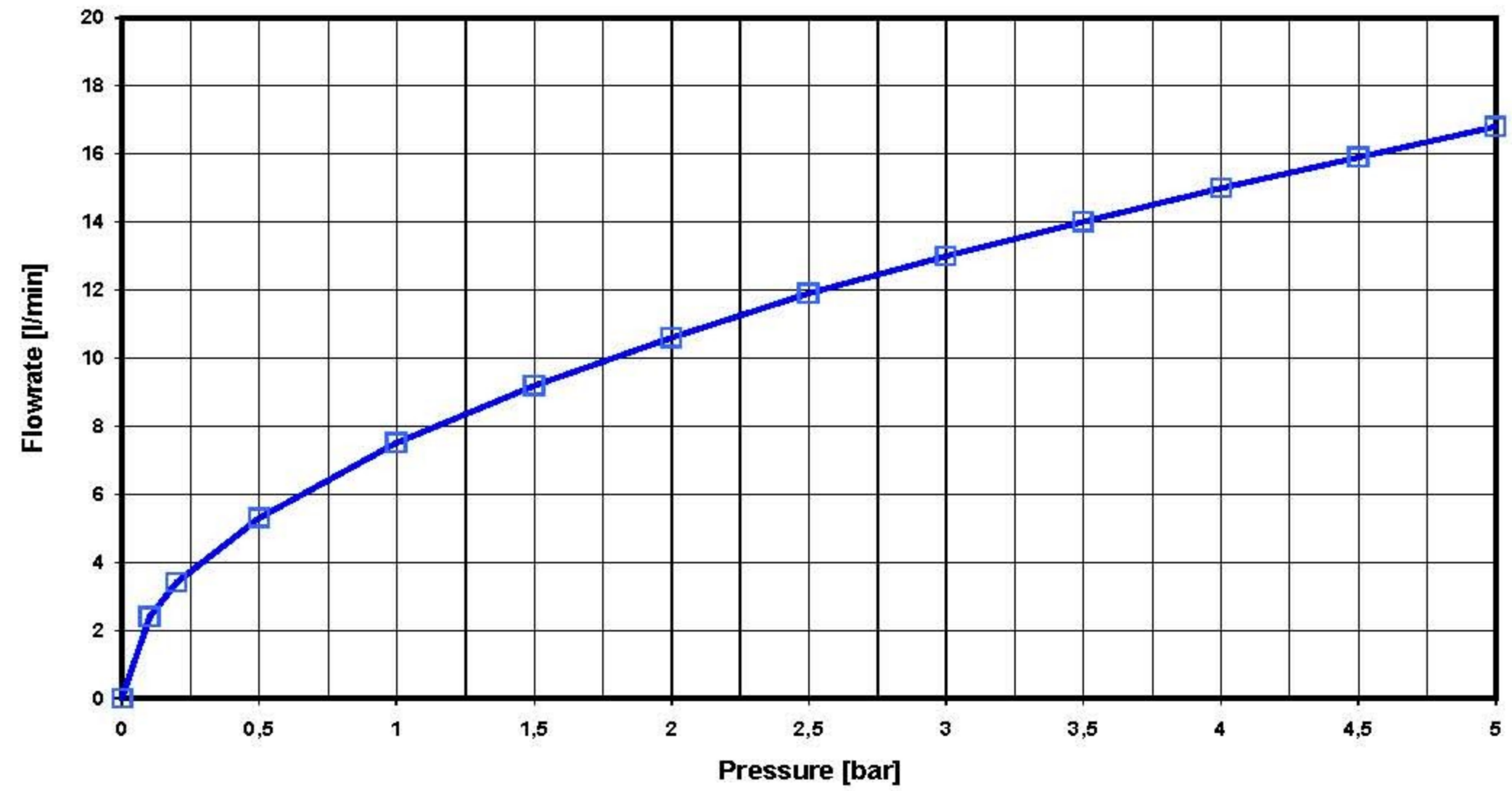
—■— Mixed water Aerator "A"
