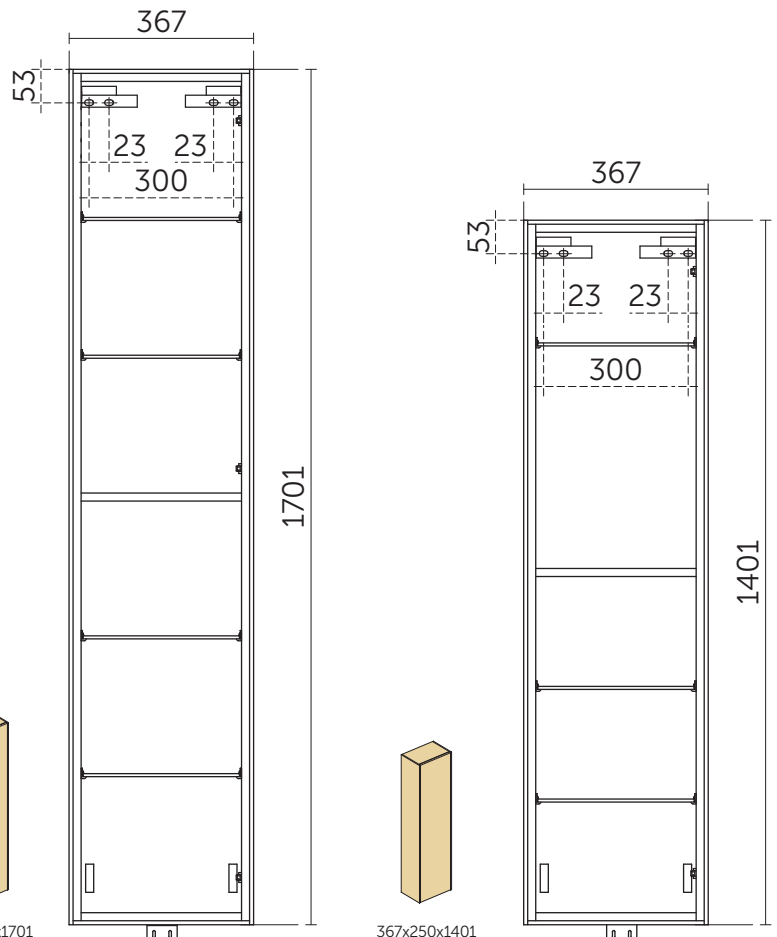
367x250x1401
