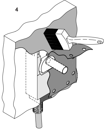
Coating - 2 nd time over rubber membrane
