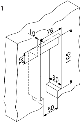
1/2" connection for copper tubes, plastic tubes (PEX pipe), or steel tubes
