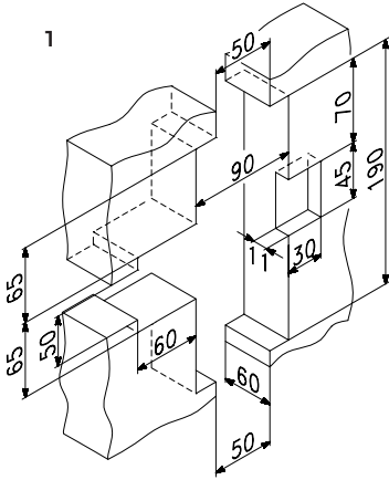
Cut-out, brickwork
