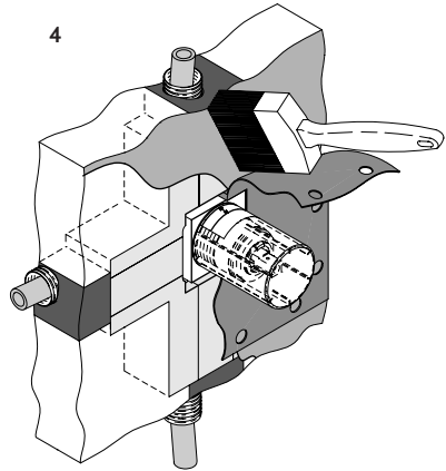
Coating - 1 st time under rubber membrane
