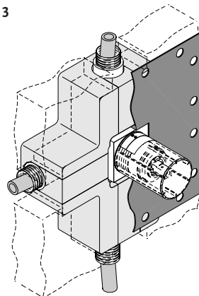
Walling up
