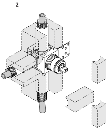
1/2" connection for copper tubes, plastic tubes (PEX pipe), or steel tubes
